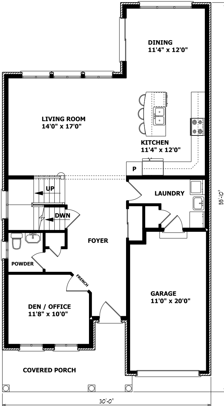
1ST FLOOR PLAN GROSS FLOOR AREA : 1111 SQ.FT.
