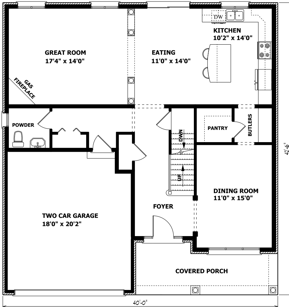
THE HUDSON 1ST FLOOR PLAN GROSS FLOOR AREA : 1176 SQ.FT.
